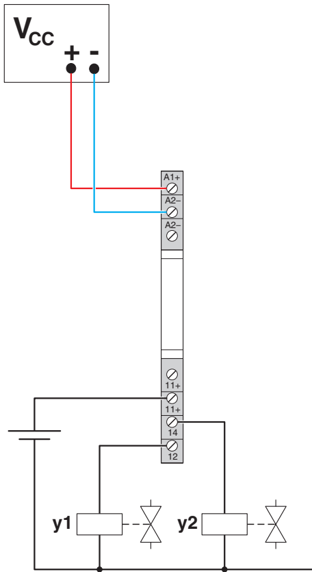
Application drawing
